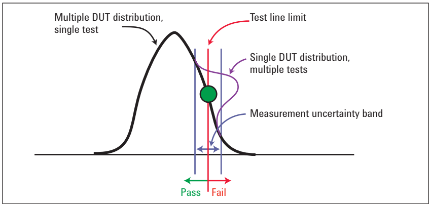
Figure 2. Test limit crossing multiple DUT single test normal distribution
